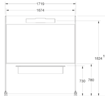
Mobile X-Line Executive for Sony BZ40 75"
